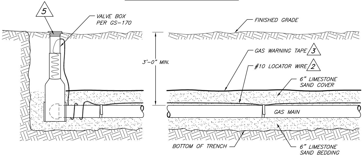
END OF GAS MAIN
