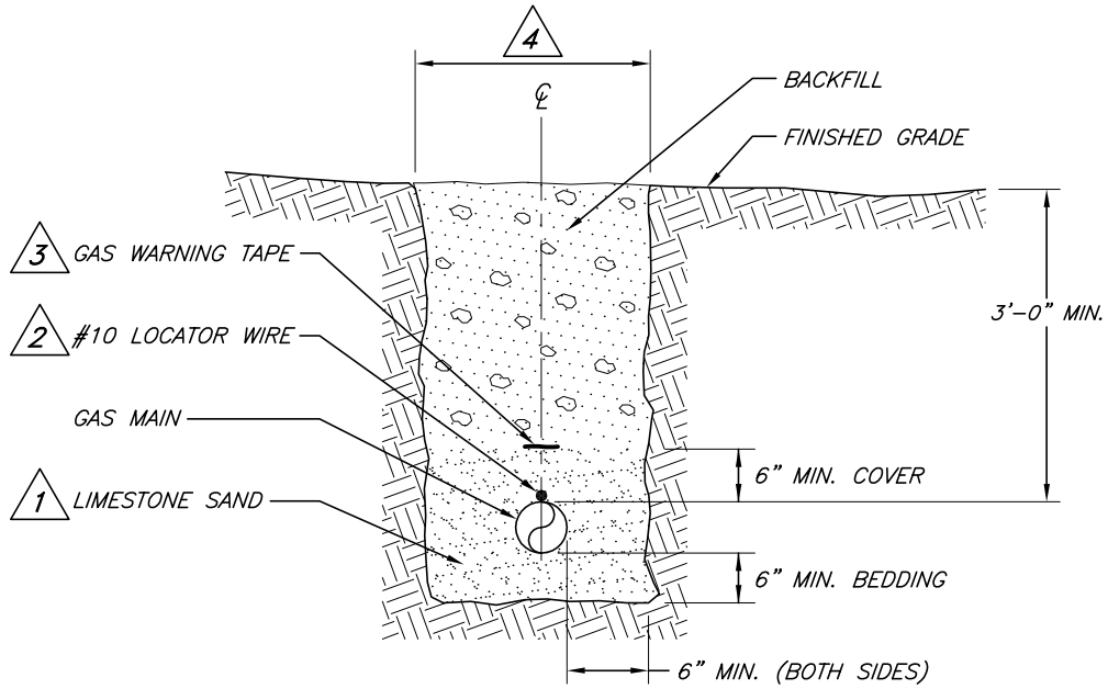
GAS MAIN TRENCH CROSS SECTION
