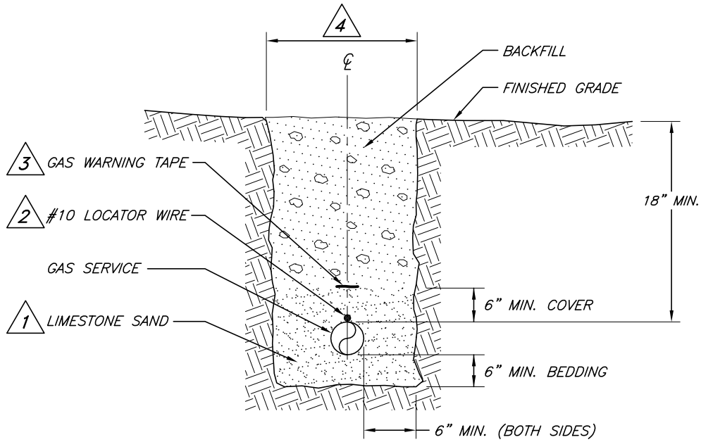
GAS SERVICE TRENCH CROSS SECTION
