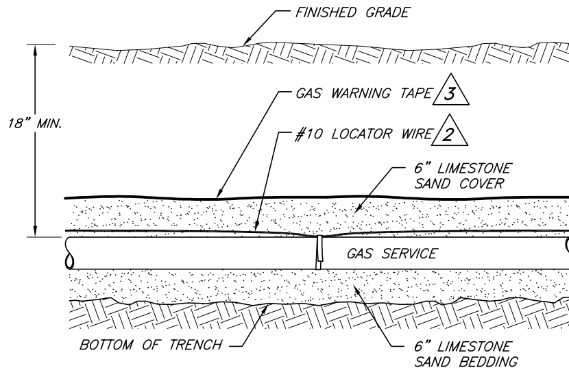
GAS SERVICE TRENCH PROFILE
