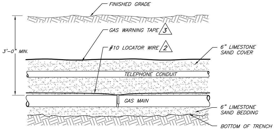
GAS/TELEPHONE JOINT TRENCH PROFILE
