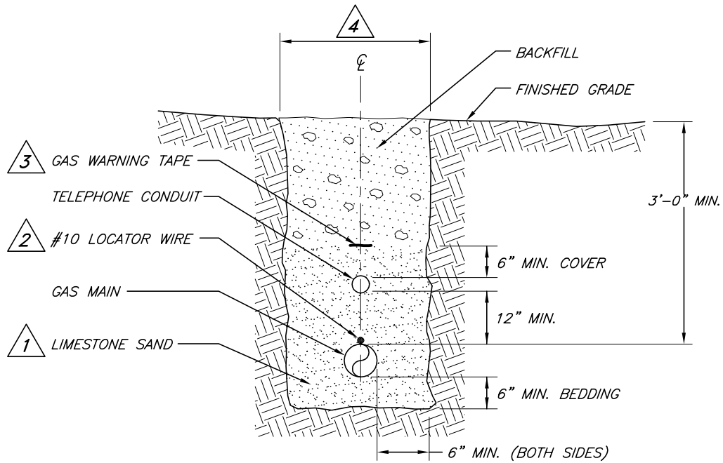
GAS/TELEPHONE JOINT TRENCH CROSS SECTION
