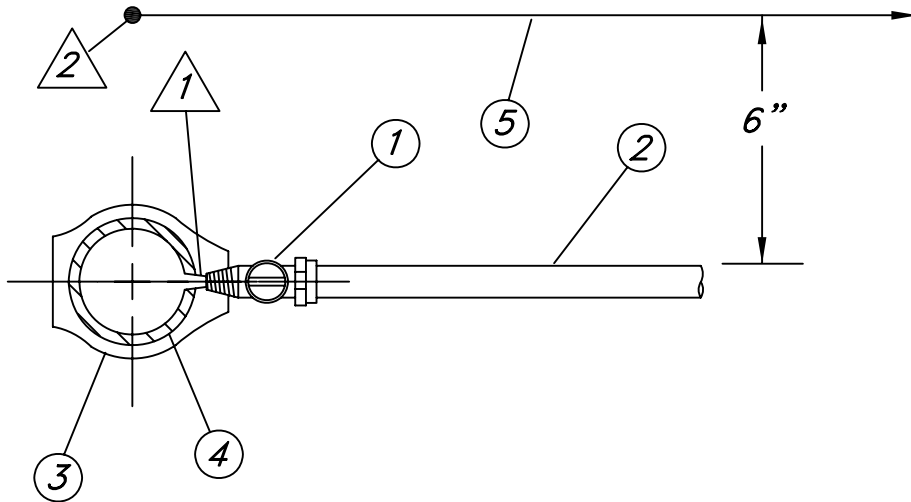
SADDLE W/CORPORATION STOP (C900 PVC MAINS)
